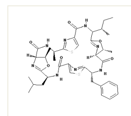
patellamide B
