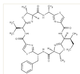
patellamide C
