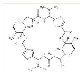
patellamide A
