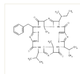
Patellamide E
